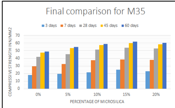
Fig11: Comparison of Strength of 3, 7, 28, 45 and 60 Days with Varying Percentage of Micro Silica For M35
