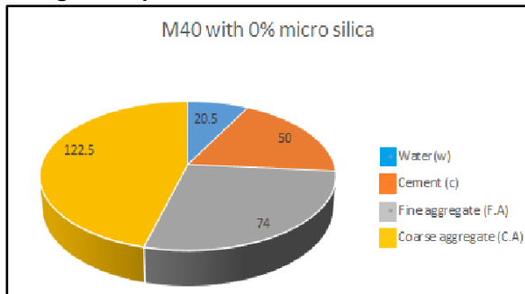
Fig3: Composition of M40 With 0% Micro Silica
