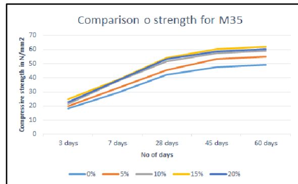
Fig10: Comparison of Strength of 3, 7, 28, 45 and 60 Days with Varying Percentage of Micro Silica for M35
