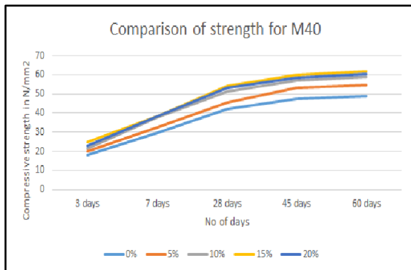
Fig12: Comparison of Strength of 3, 7, 28, 45 and 60 days with Varying percentage of micro silica for M40
