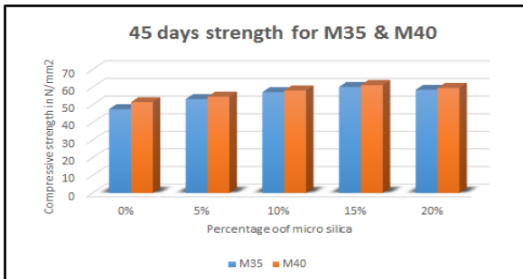
Fig 8: 45 Days Compressive Strength of M35 with Varying Percentage Oof Micro Silica
