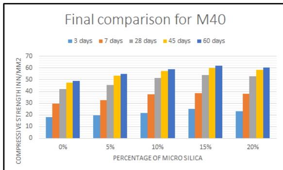
Fig13: Comparison of Strength of 3, 7, 28, 45 and 60 days with varying Percentage of Micro Silica for M40.
