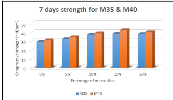
Fig6: 7 Days Compressive Strength of M35& M40 with Varying Percentage of Micro Silica.
